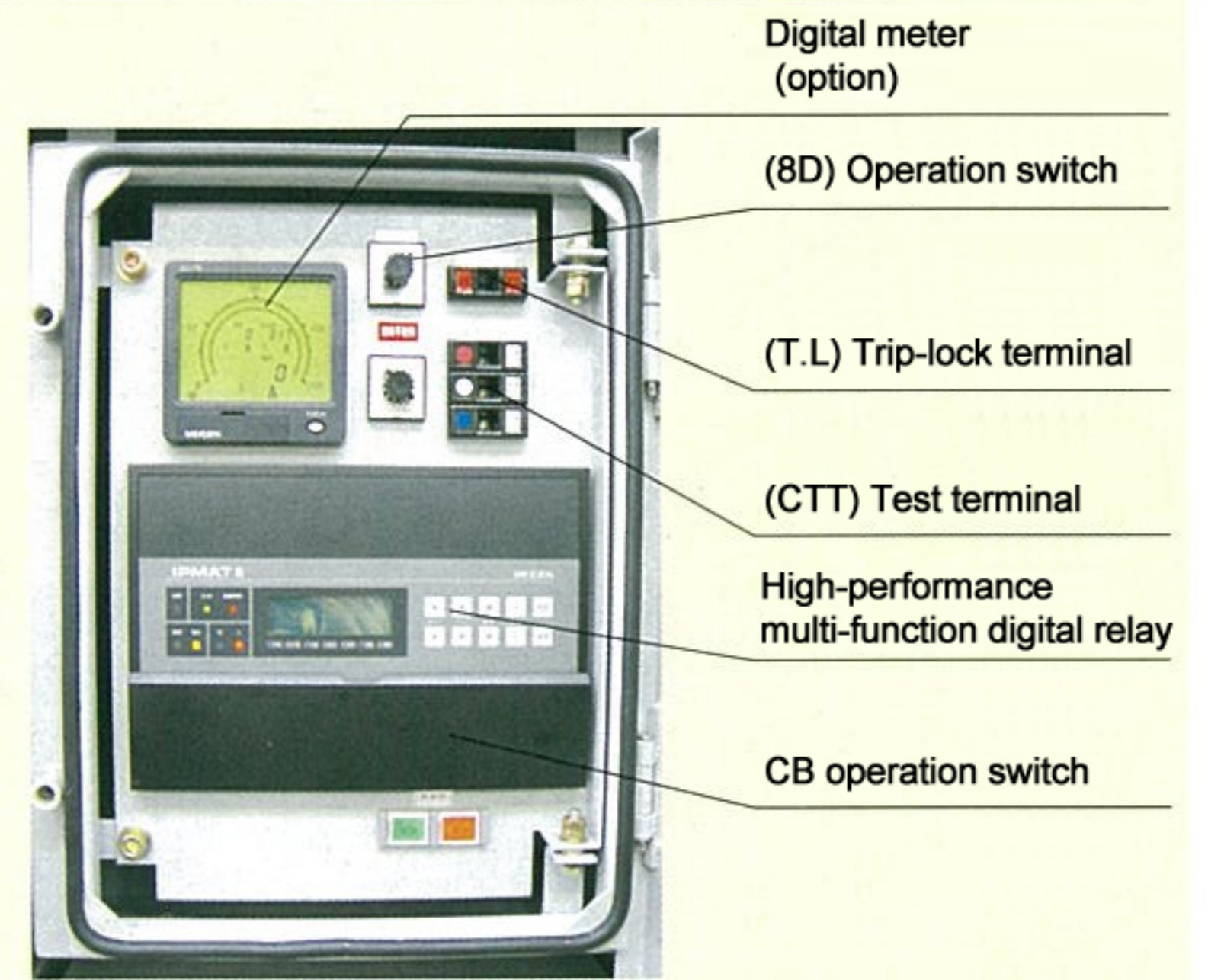
Monitoring and control box incorporating a protective relay and a meter for measurement
