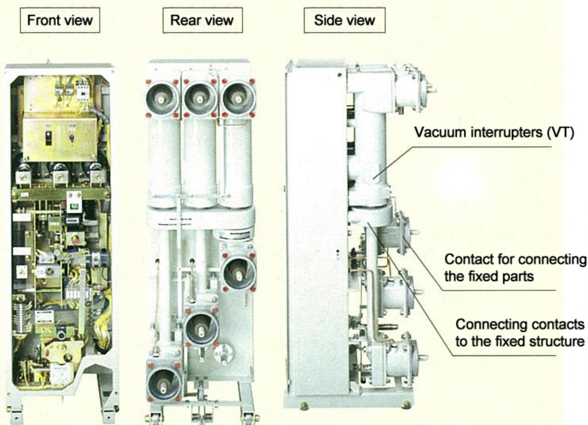
Draw-out unit incorporating the main circuit components (such as VCB, CT, ZCT, VT, and EVT) (All units with the same specifications are interchangeable.)
