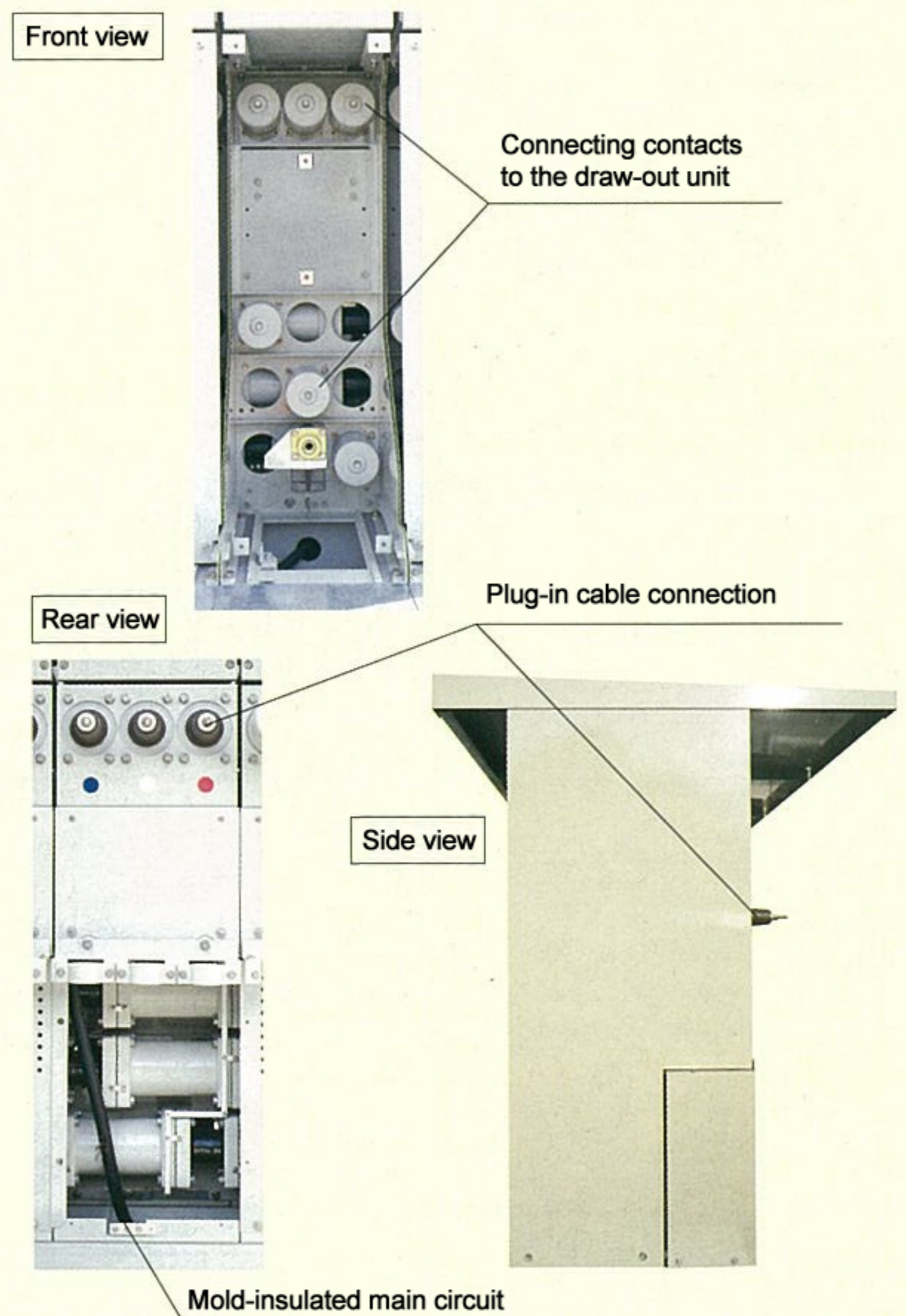
SIS main body housing the molded main circuit
