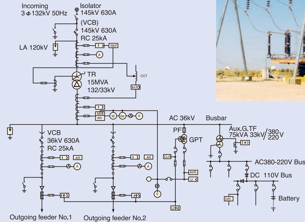
Single Line Diagram for the Compact Mobile Substation
